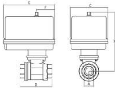
IP-Series 2-Piece Brass Ball Valves
